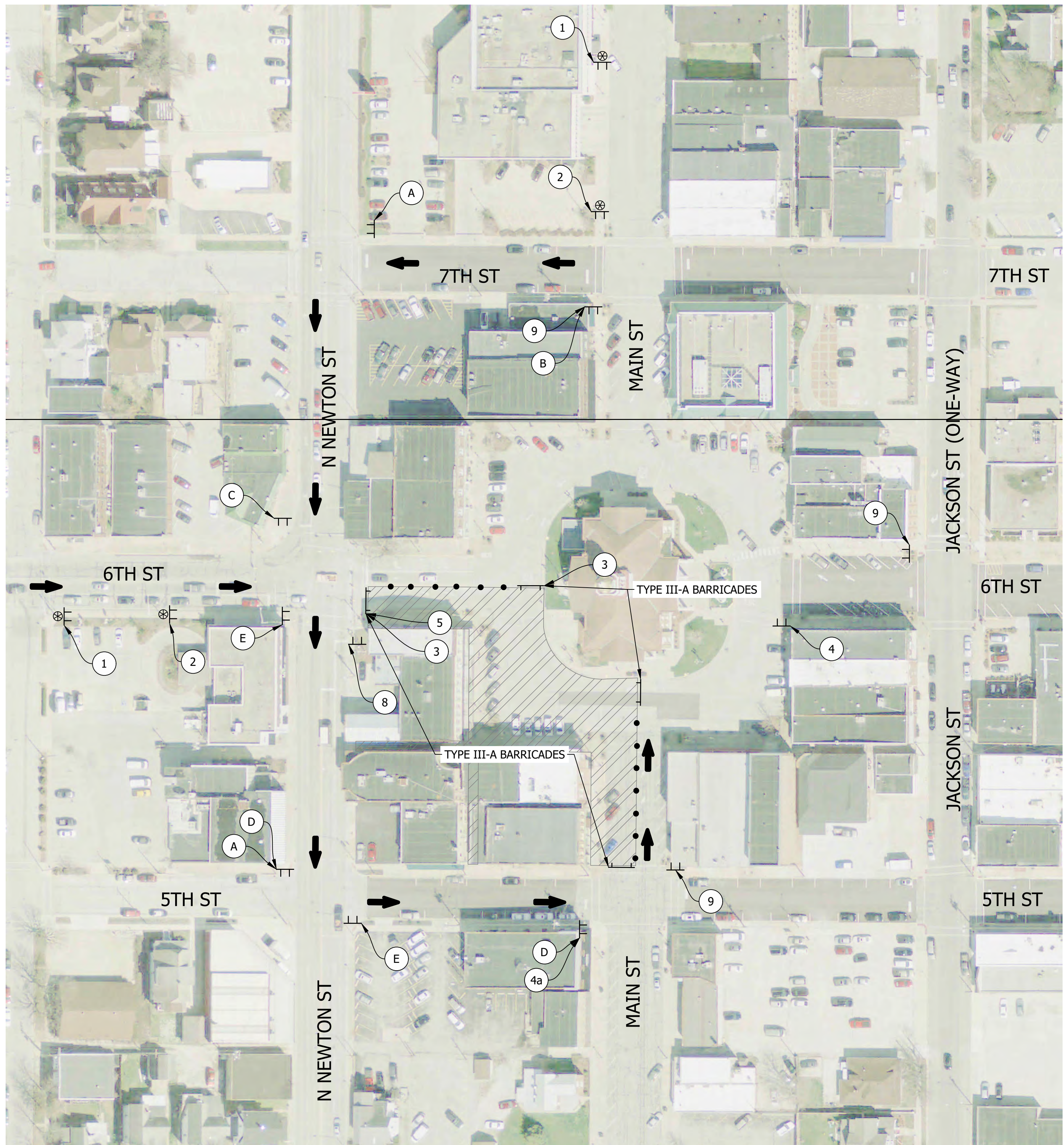
Detour Route "South Main/East 6th" Phase IV Scale: 1" = 60'-0"
